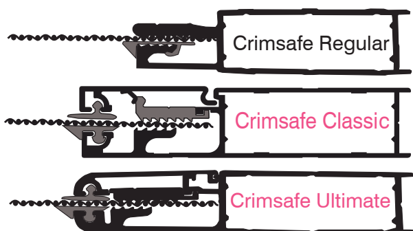
Cross section of mesh and frame featuring the New Carbon Fibre Screw-clamp 'clip' system.
